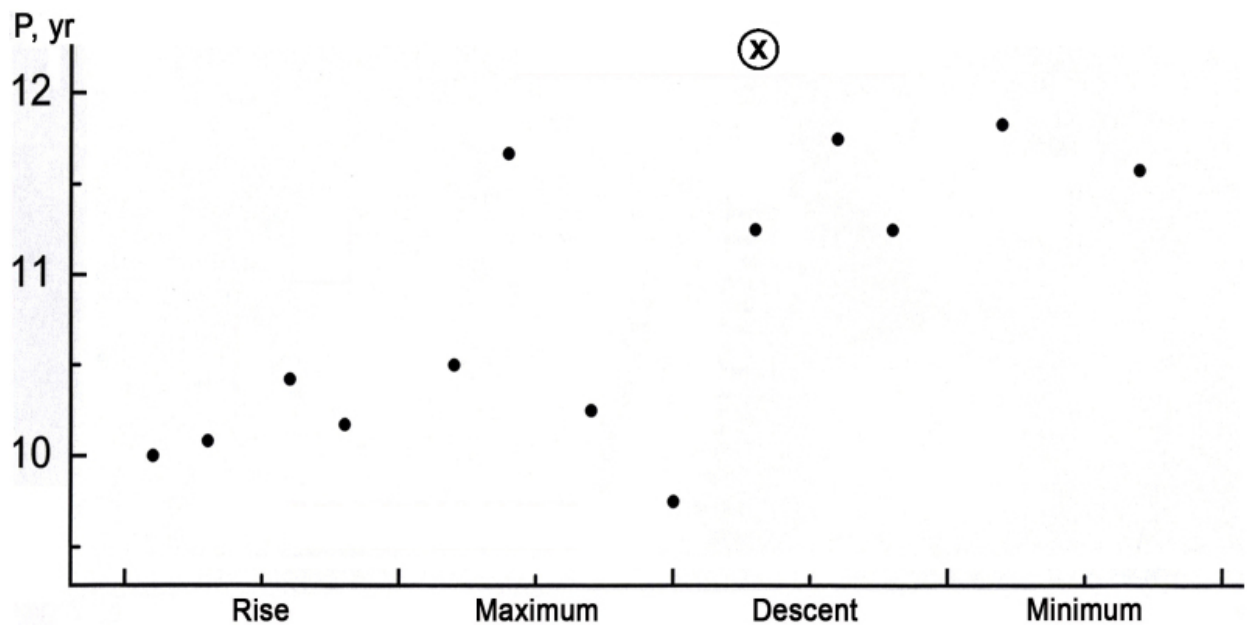
Fig. 4. Dependence of the duration of the 11-year cycles of the sunspot activity ( P ) on the phase of bicentennial cycle ( X - 23rd cycle). Plotted on the Y-axis is the duration "short" cycles; plotted on the X-axis - phase of bicentennial cycle.
