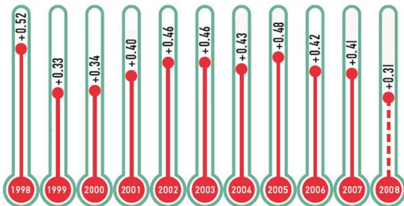
Fig. 11. Observed stabilization of temperature for the last ten years and its tendency to drop in 2006-2008.
